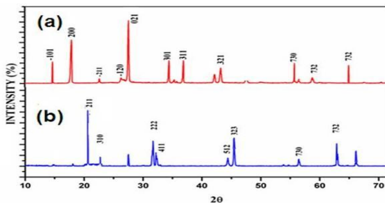
Fig. 5: The XRD pattern of struvite obtained from Alpinia purpurata stem in the gel method (a) without any additive (b) with the 1.00% of methanol extract.
