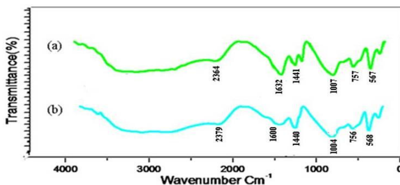
Fig. 4: The FTIR spectra of struvite obtained from Alpinia purpurata stem in the gel method (a) without any additive (b) with the 1.00% of methanol extract.
