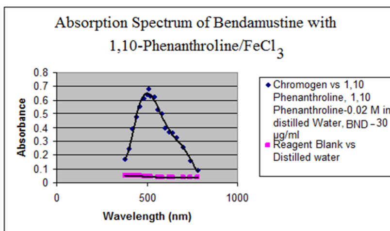
Figure 2: Absorption spectrum of Bendamustine hydrochloride.
