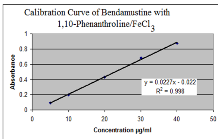
Figure 1: Calibration Curve of Bendamustine hydrochloride with 1,10 phenanthroline.
